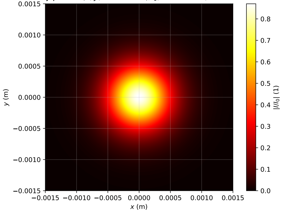
Intensity profile I(x, y, z = 1.831m)/I_0 , Pin=0.5Pcr, artificial time
